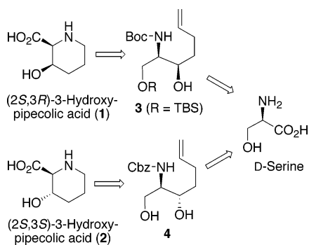
FIGURE 1. Retrosynthetic strategy and approach.
